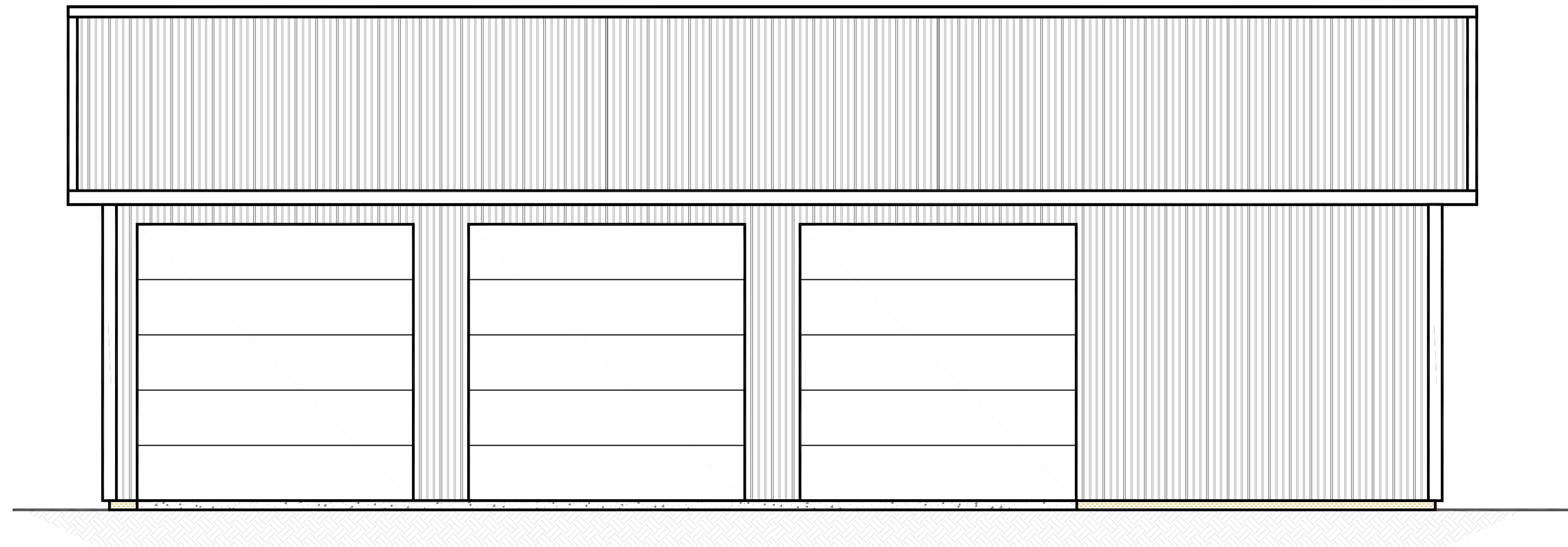
FRONT EAVE VIEW
