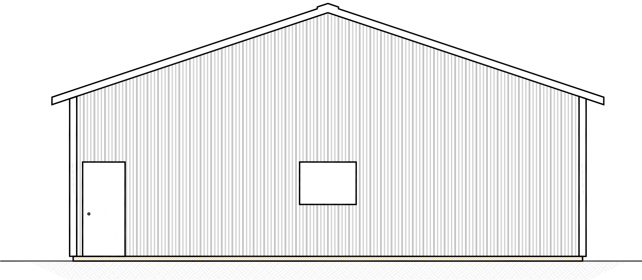
RIGHT GABLE VIEW
